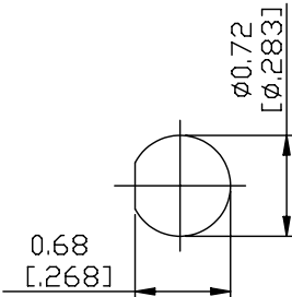
MOUNTING HOLE
