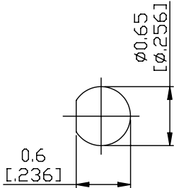
MOUNTING HOLE
