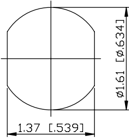
MOUNTING HOLE
